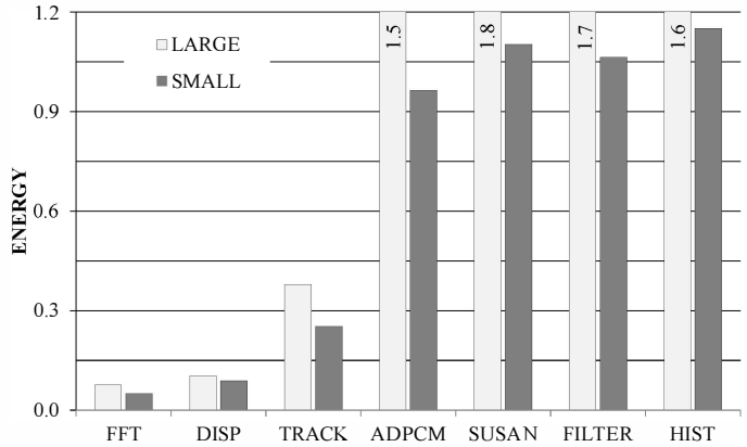
Figure 7: Comparing the benefits of LARGE (L0X:8KB,L1X:256KB) vs SMALL (L0X:4KB,L1X:64KB)
