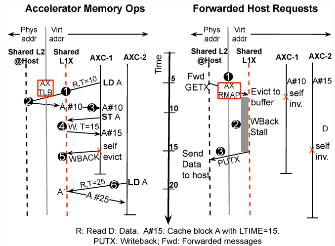
Figure 4: Left: ACC protocol servicing requests from accelerator and interaction with MESI. Right: ACC Protocol servicing forwarded requests from MESI.
